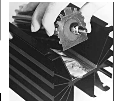
Heat-Away™ 638 used as a heat transfer grease between a high temperature ballast resistor and an aluminum heat sink.
